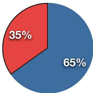
Cations
