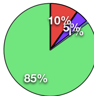
Anions
